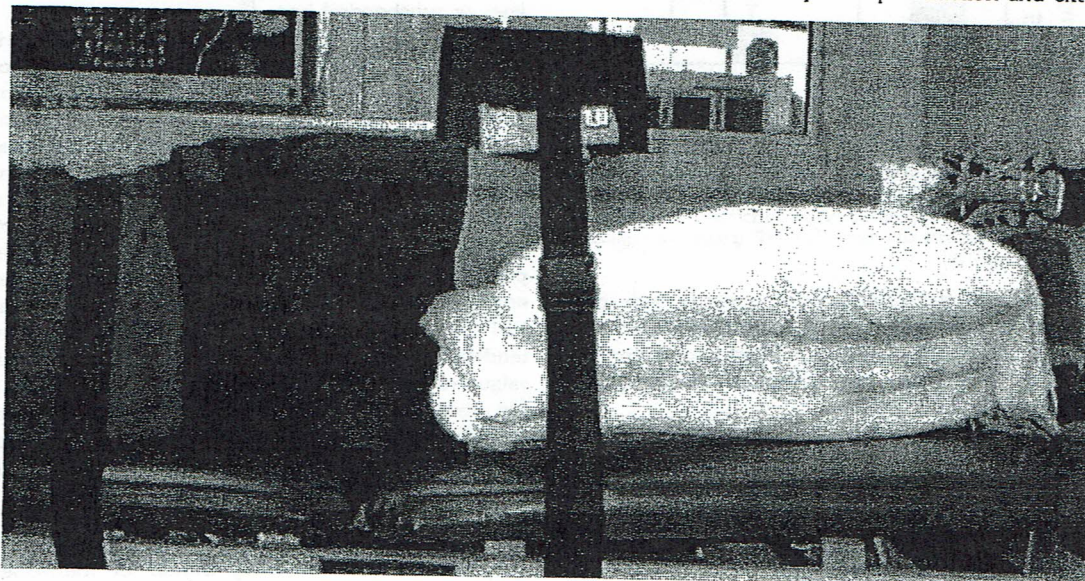
FIGURE 1. Isometric strength testing of hip abduction using straps and hand-held dynamometer.
